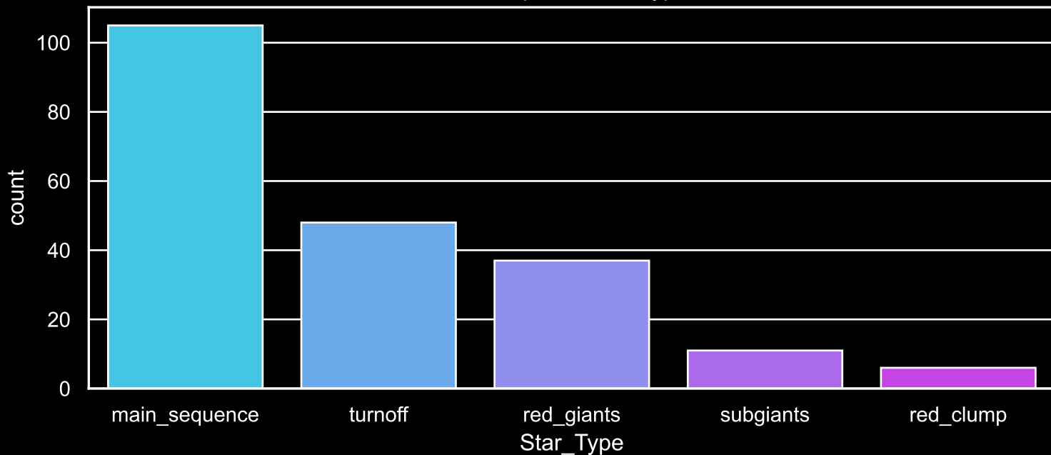
Field [16] Count plot of Star Type
