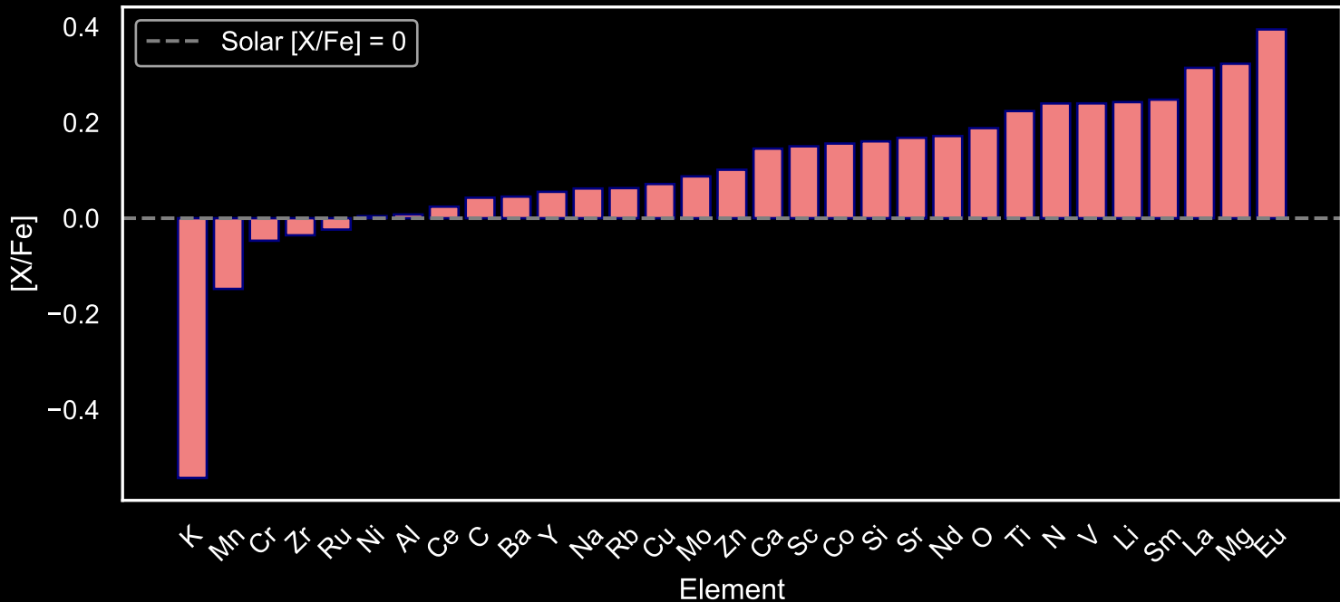
Abundance Pattern for GALAH Red Giants: Star Field [16] (N=43)
