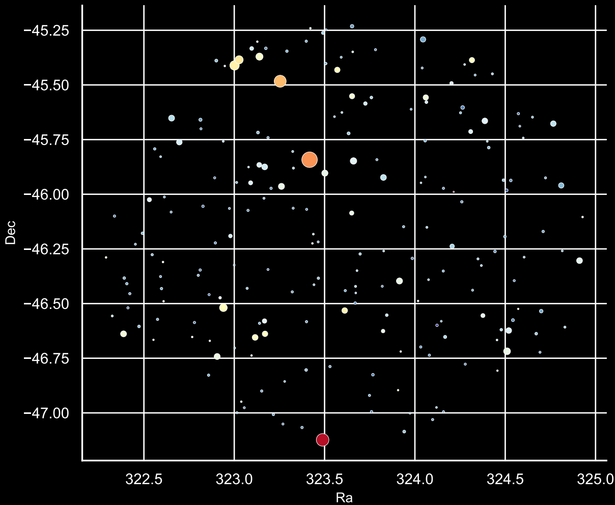
Field [16] Ra [323.58] Dec [-46.17] Stars: 207
