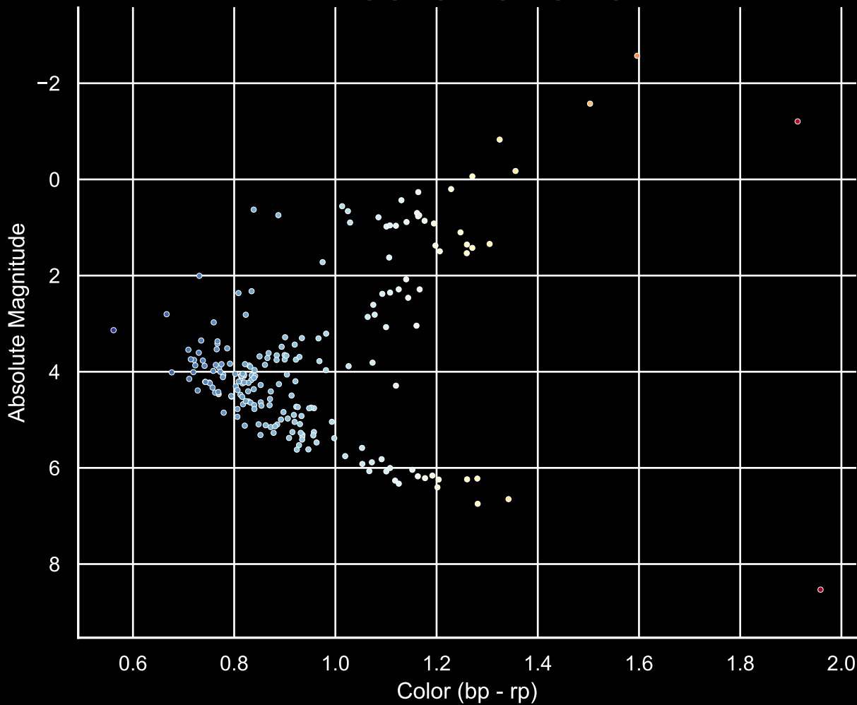
GALAH Hertzprung-Russell Diagram Field [16] Ra [323.58] Dec [-46.17]
