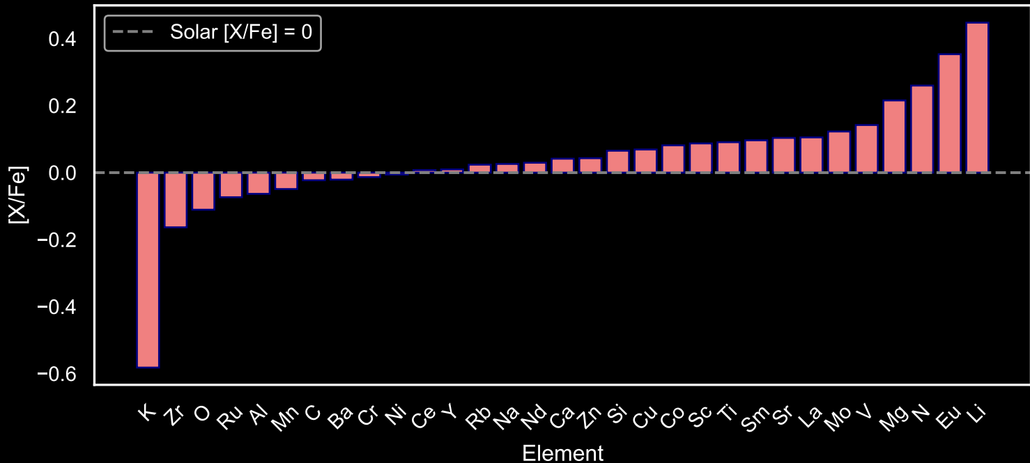
Abundance Pattern for GALAH Star Field [16] (N=207)
