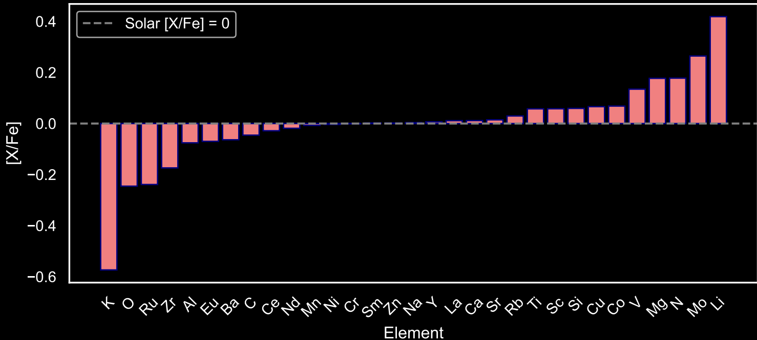
Abundance Pattern for GALAH Main Sequence Stars: Star Field [16] (N=105)
